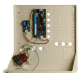
ATS1500AV-IP-LM 8-32 zones, boîtier grand, IP, SES-CH
